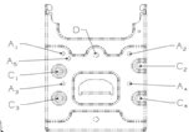
ENGINE MOUNTING HOLE DIMENSIONS ENGINE MOUNTING PLATE DIMENSIONS ONLY
