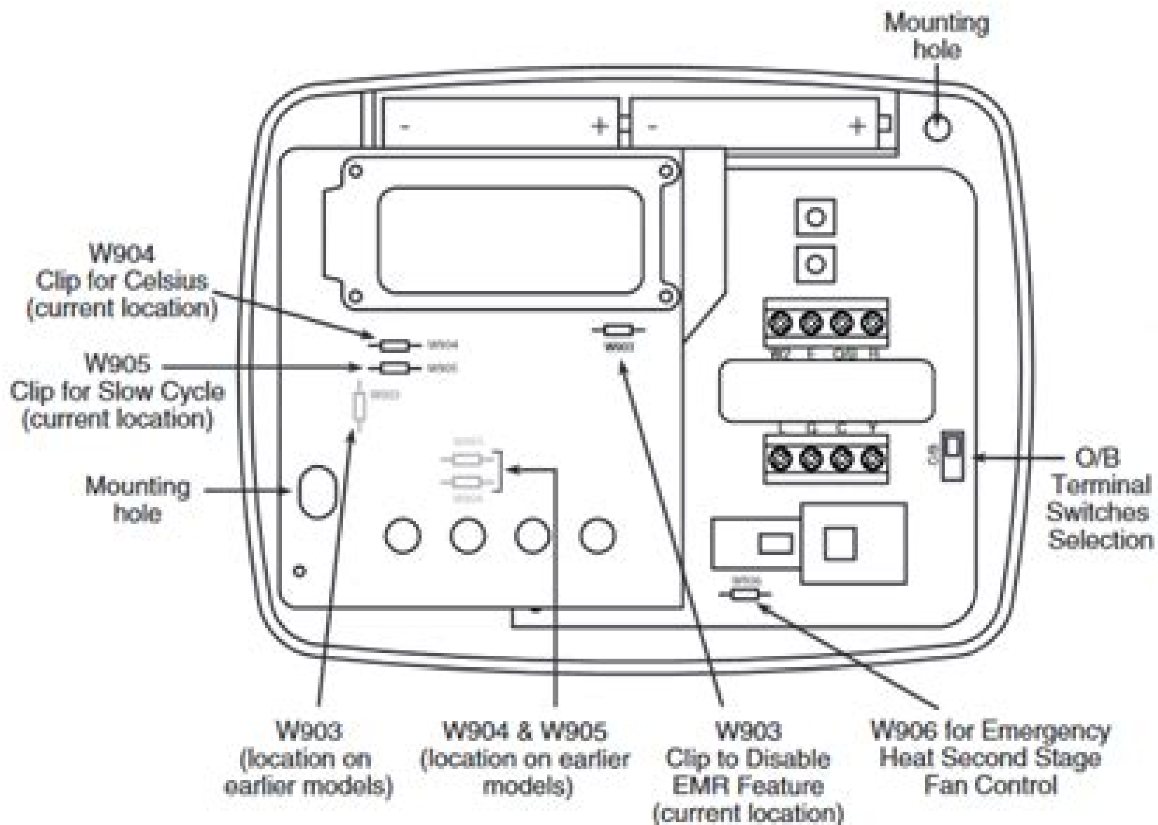
Figure 1. Thermostat base
