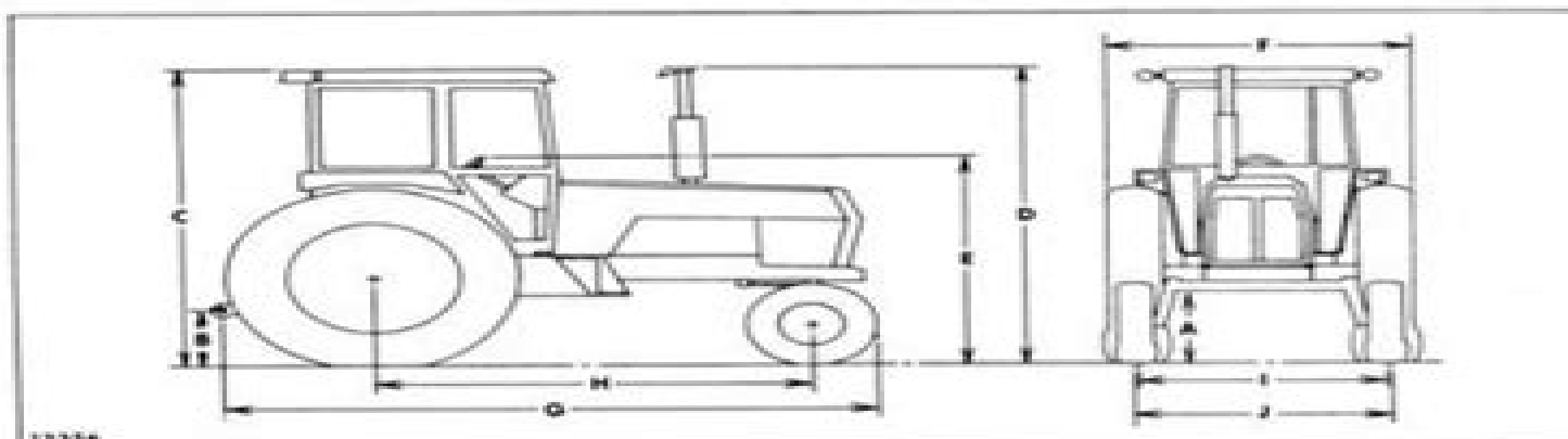
Fig. 4 — Tractor Dimensions
