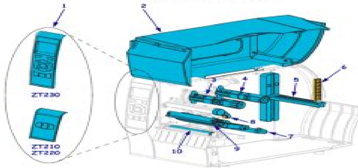
Figure 1 • Printer Components
