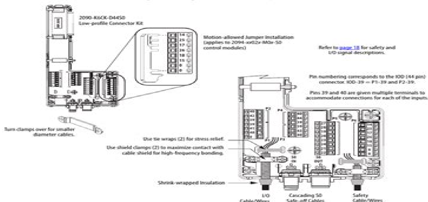
Figure 2 - Making 2090-K6CK-D4450 Safety Connections
