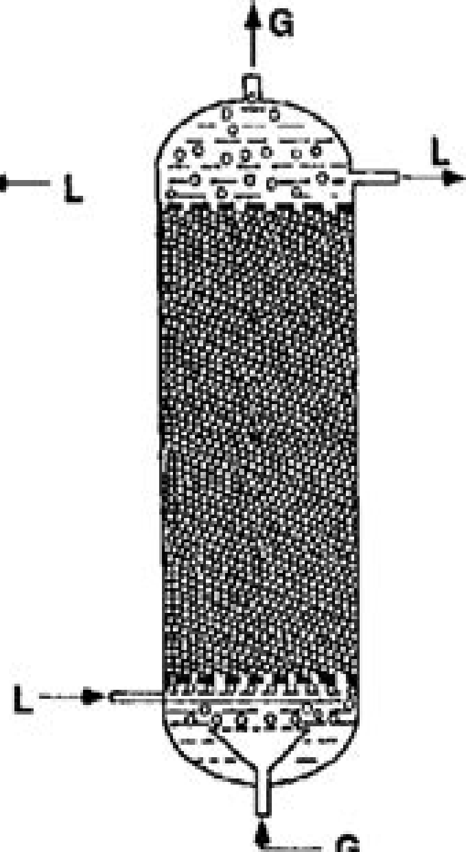
(c) Packed - Bubble Flow Cocurrent upflow
