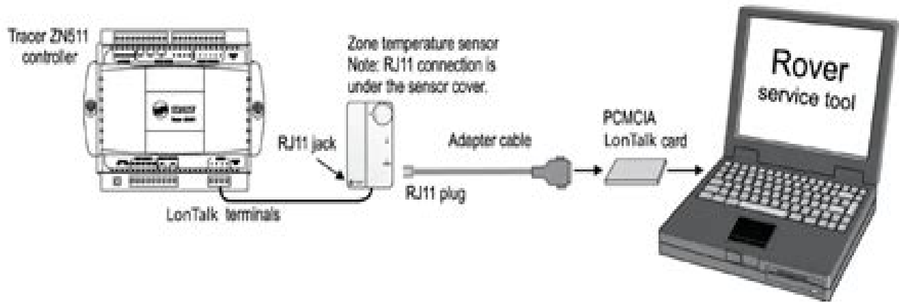
Figure 3. Connecting to a LonTalk controller through a zone sensor
