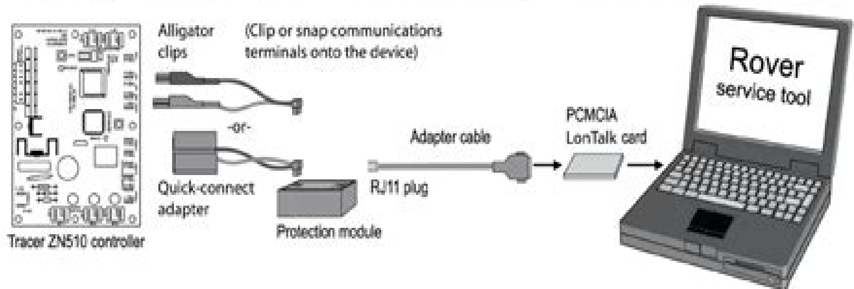
Figure 4. Connecting to a LonTalk controller using alligator clips or quick-connect adapter
