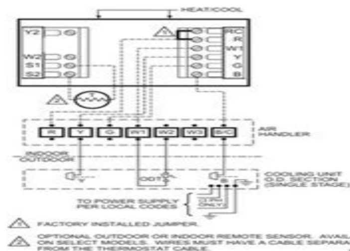
Fig. 5. Typical hookup of single-stage heat and cool system with single transformer (1H/1C).
