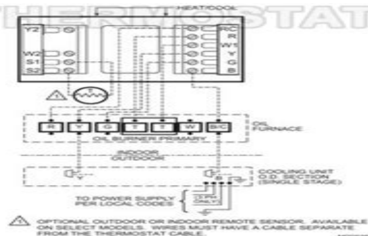
Fig. 6. Typical hookup of single-stage heat and cool system with two transformers (1H/1C).
