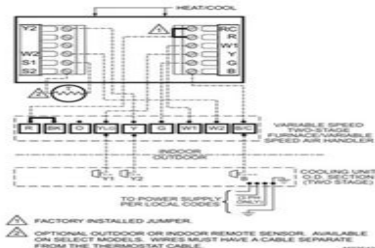
Fig. 7. Typical hookup of two-stage indoor and two-stage cooling unit in a single transformer system (2H/2C or 2H/1C or 1H/2C).
