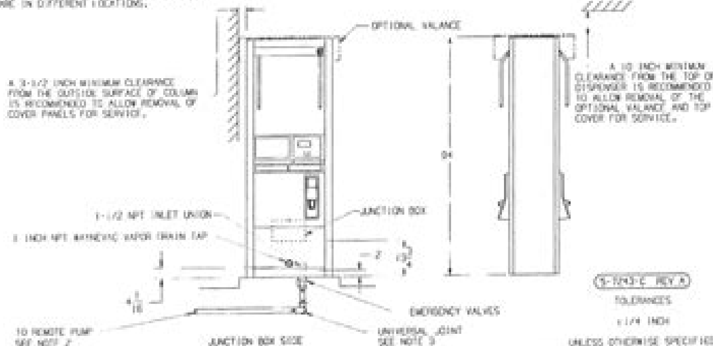
BASE DIMENSIONS
