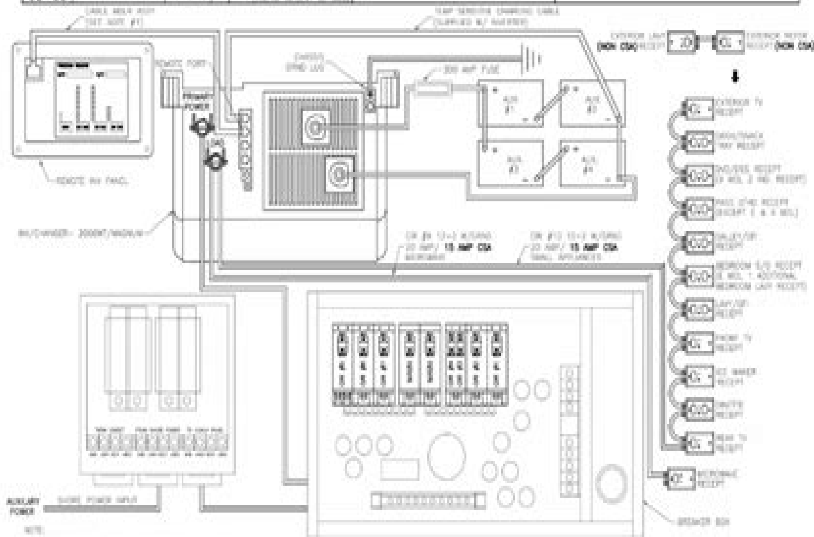
2000W INVERTER/CONVERTER WIRING INFO
