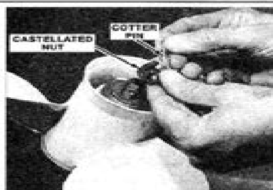
Fig. 73 Most Yamaha props are secured by a nut and cotter pin
