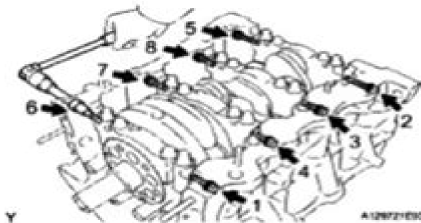
Fig. 275: Locating Connecting Rod Bearing Cap Bolts Courtesy of TOYOTA MOTOR SALES, U.S.A., INC.
