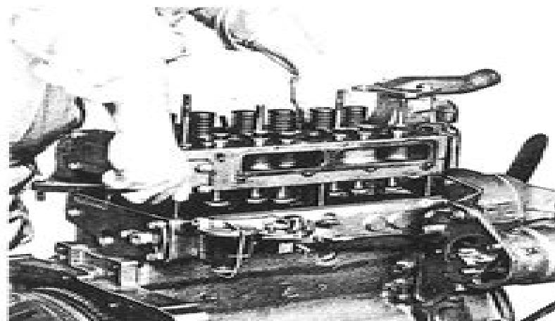
Fig. 9 - Removing or Installing the Cylinder Head
