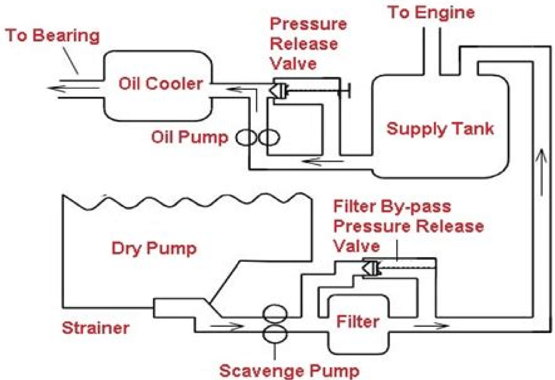
Dry Sump Lubrication System
