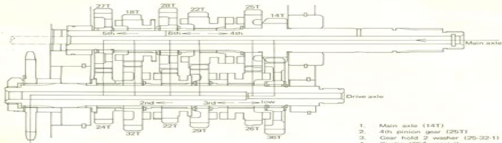
Sectional View of Transmission (6-Speed) Fig. 3-13-3
