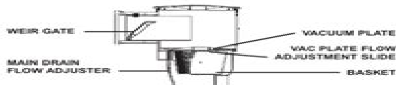
* Figure 2: SP5000 Skimmer Box (side view)
