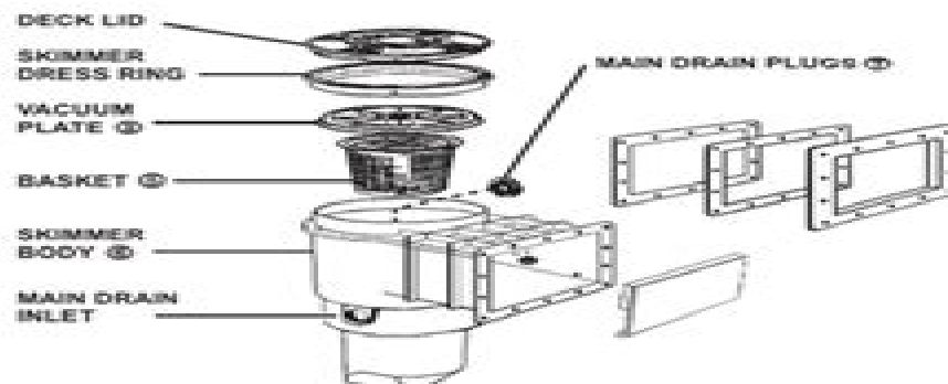
* Figure 3: S75 and Supaskimmer Skimmer Boxes
