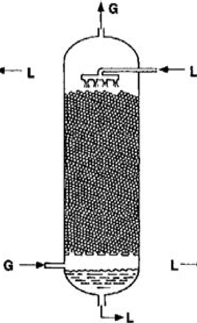
(b) Trickle - Bed Countercurrent flow
