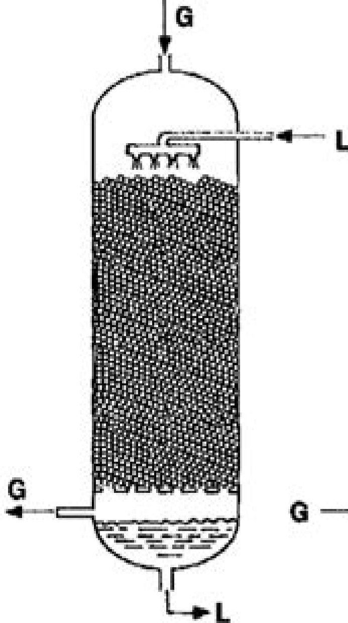
(a) Trickle - Bed Cocurrent downflow
