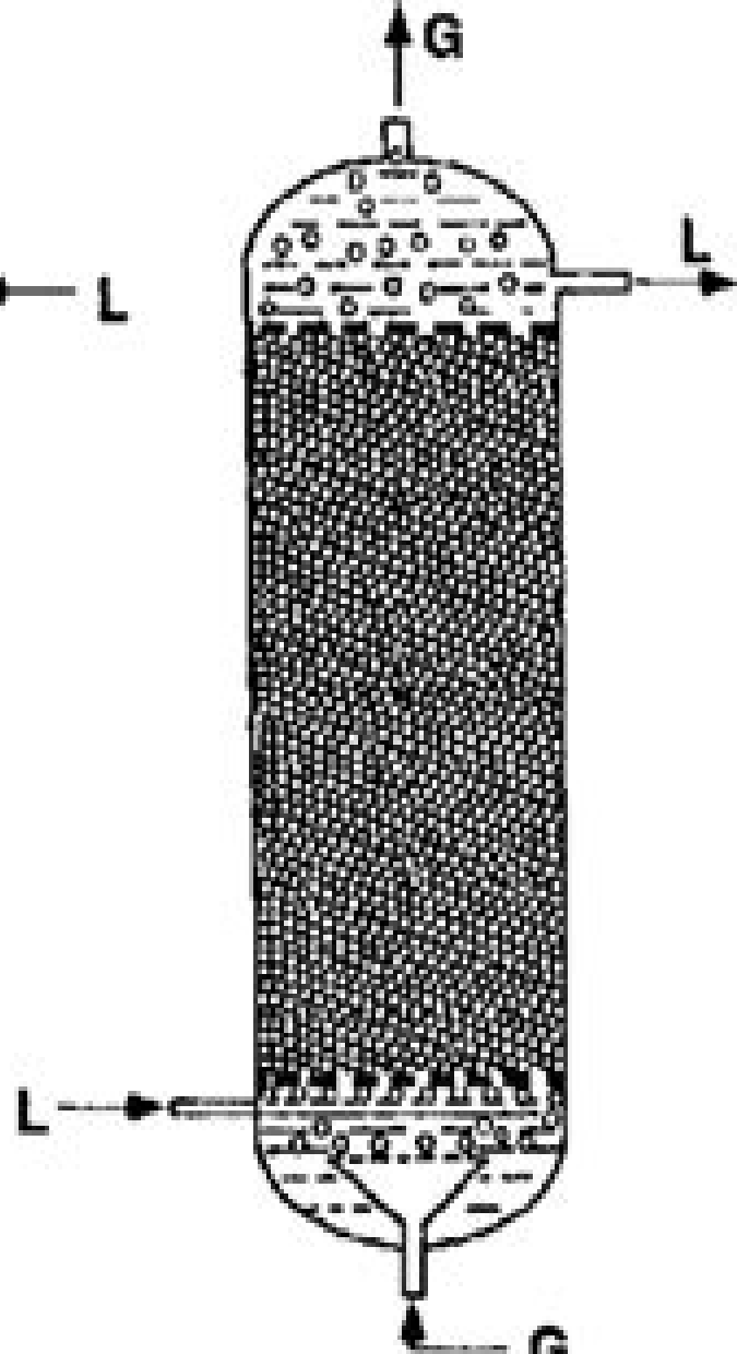
(c) Packed - Bubble Flow Cocurrent upflow
