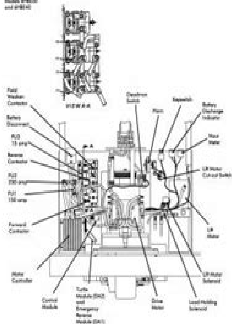
Figure 1.12 Models 4HBE30 and 4HBE40 Electrical Wiring
