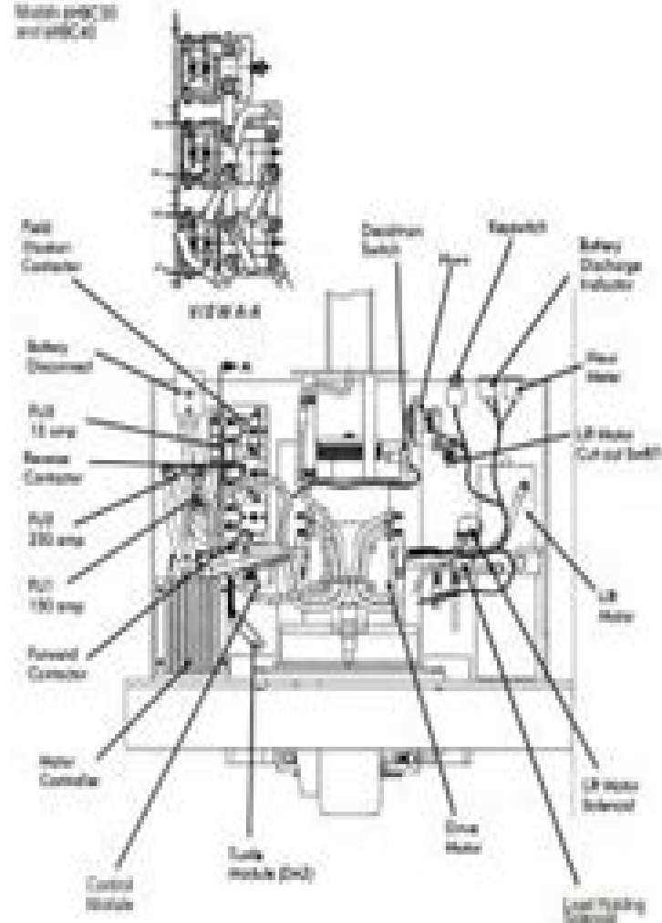
Figure 1.13 Models 4HBC30 and 4HBC40 Electrical Wiring
