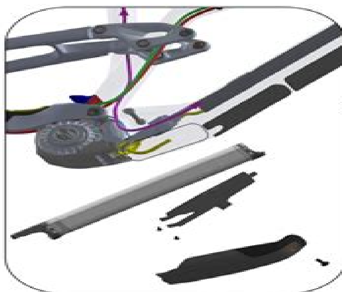
Dropper post cable routing (See pages 9 and 11 for part information)
