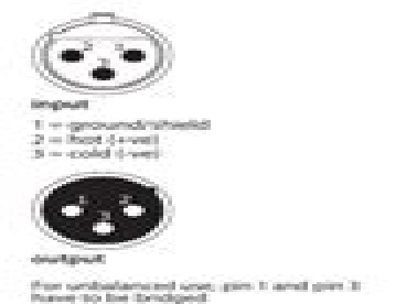
Fig. 4.1: XLR connections
