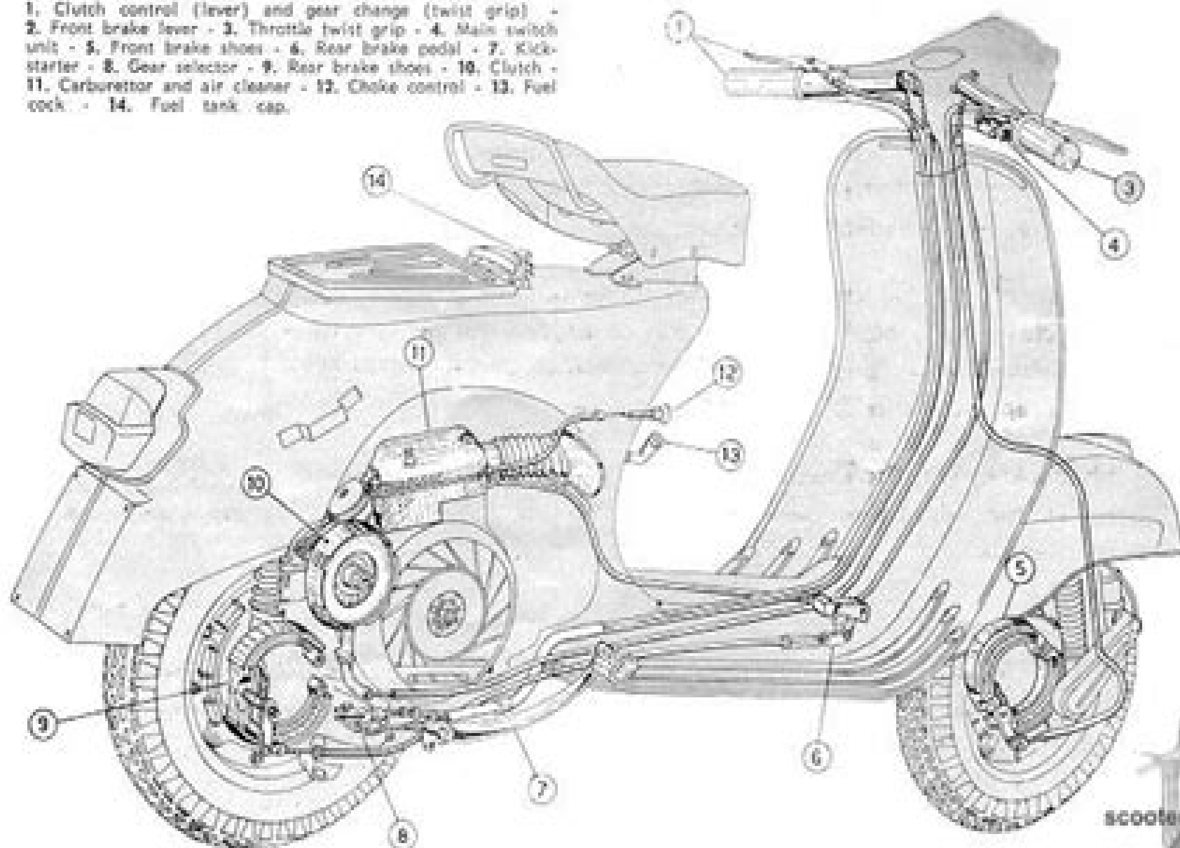
Fig. 2 - Installation of controls and transmissions
