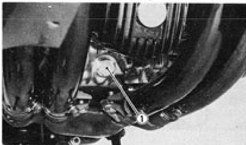
1. Drain plug
