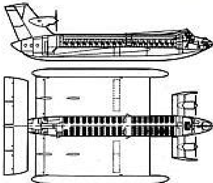
Fig. 1.17 Russian WFO type "Molot-2"
