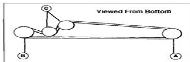
Figure 39. Drive Belt Routing - Hydro Models A. Engine Pulley B. Transmission Pulley C. Idler Pulley
