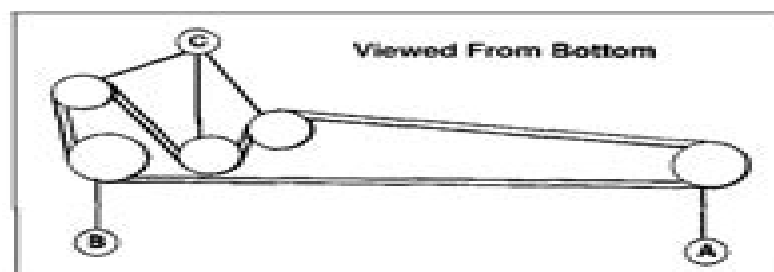
Figure 38. Drive Belt Routing - Gear Models A. Engine Pulley B. Transmission Pulley C. Idler Pulley
