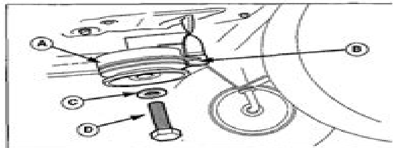
Figure 37. PTO (Electric Clutch) Assembly A. PTO B. Sleeve C. Washer D. Capscrew
