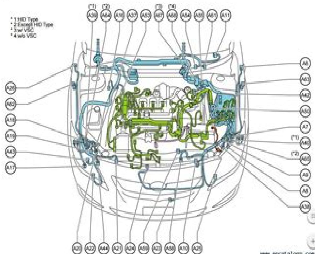
Position of Parts in Engine Compartment (4D 5D 14D 17V)
