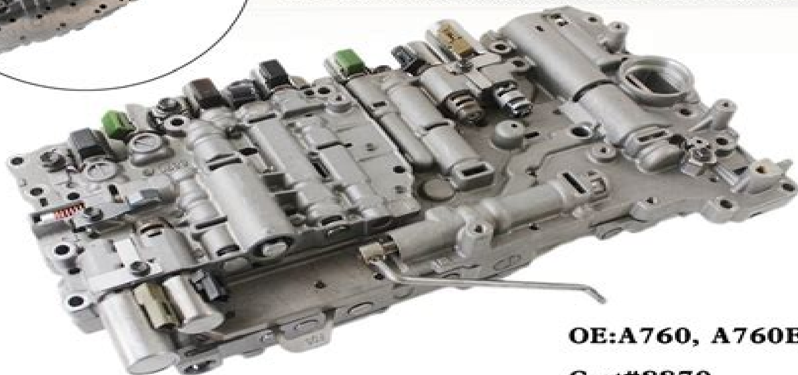
A760 A760E Transmission Valve Body W/9 Solenoids Casting#8870 For Toyota Sequoia
