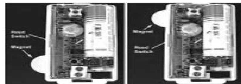
Figure 1. Acceptable magnet locations for a wall mounted UFT.
