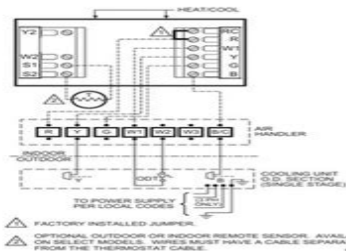
Fig. 5. Typical hookup of single-stage heat and cool system with single transformer (1H/1C).
