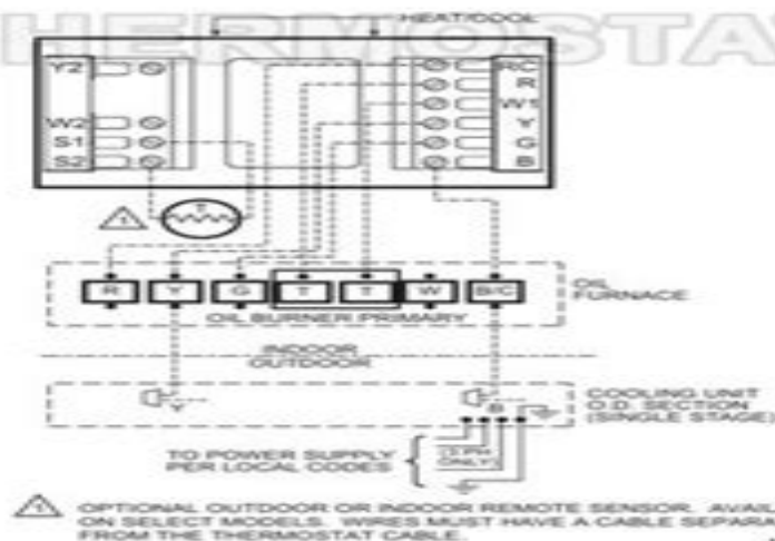
Fig. 6. Typical hookup of single-stage heat and cool system with two transformers (1H/1C).
