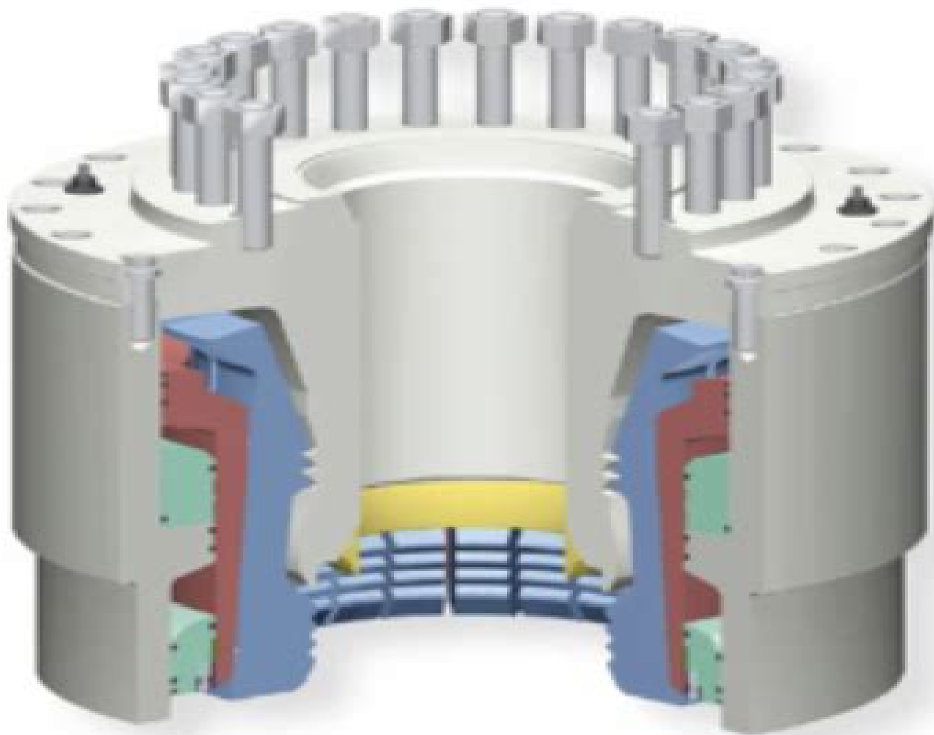
H4 CONNECTOR WITH STUDDED TOP
