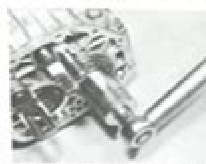
6.24a Tighten the primary (where applicable) and secondary shaft nuts ...
