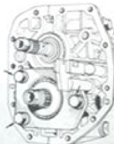
Fig. 6.21 Refit the bearing seat plate onto the rear face of the 365 gearbox (Set 6)
