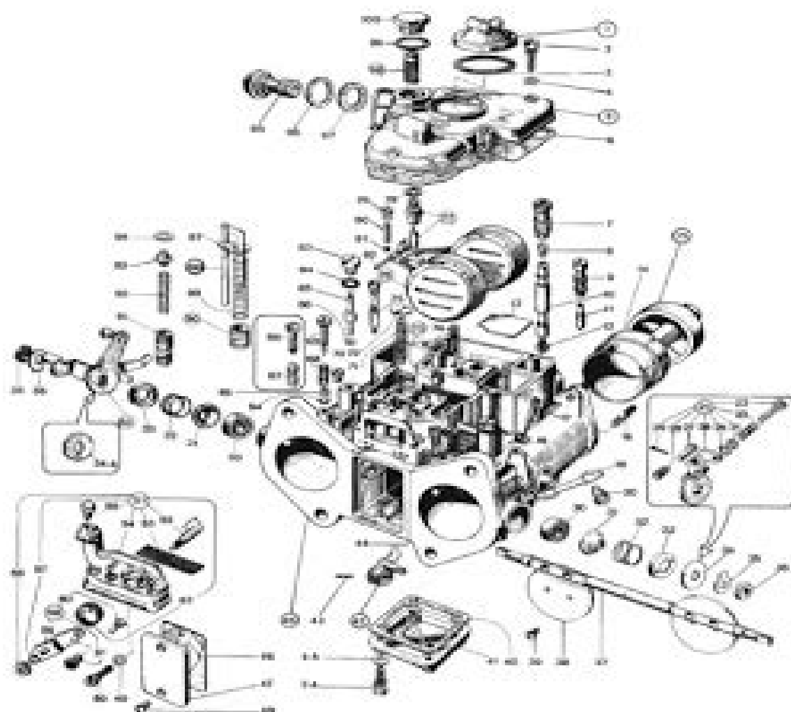
Fig. 7 - Exploded view of carburetor
