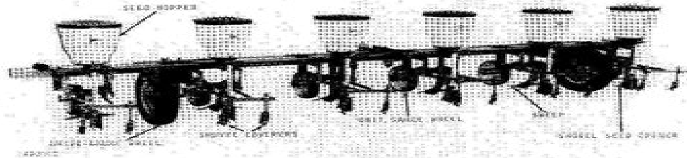
6-Row 6100 Planter with 4-Inch Chevron Tread Unit Gauge Wheels 6100 Series Planters Manufactured (1973- )
