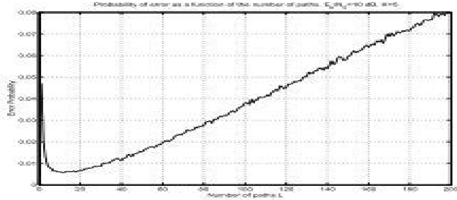
Figure 3.2: Probability of error as a function of the number of paths for \mathcal{E}_s/N_0 = 10\text{dB} and K = 5 .
