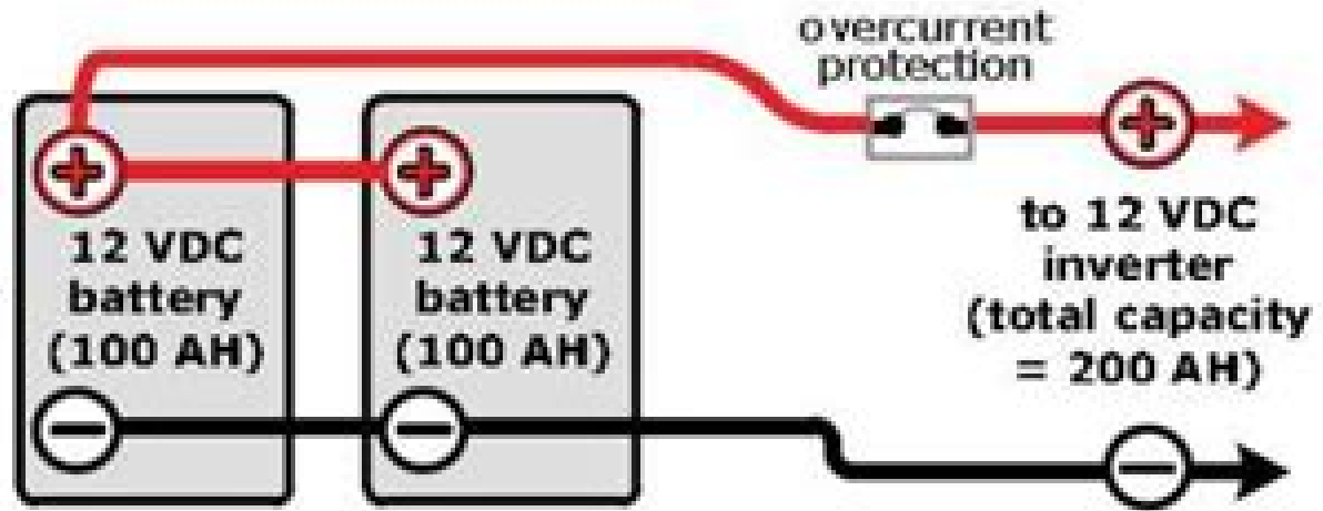
12-volt battery bank (parallel two 12-volt batteries)
