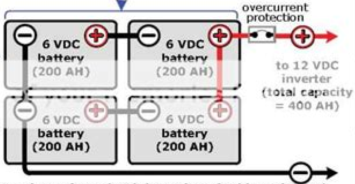
12-volt battery bank (two strings of two 6-volt batteries wired in series and connected in parallel)
