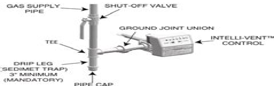
Figure 1. Typical gas connection
