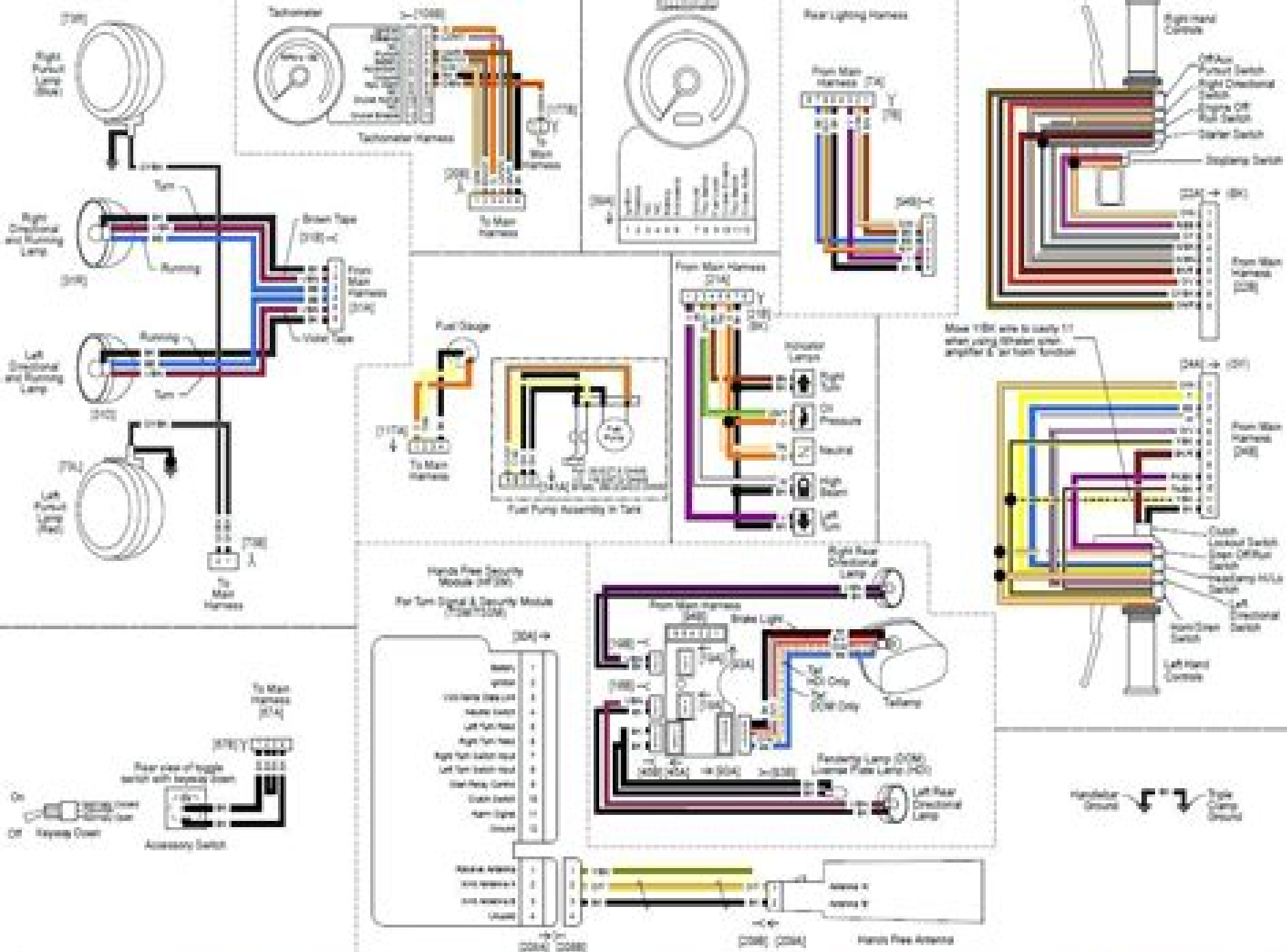
Figure A-15. Handfree Switches, Indicator Lamps, Tail Lamp, Power Lamps, Directional Lamps, Accessory/Boost Switch, Tachometer/Tachometer and IFM Antenna, 2008 FLTP and FLTPS, DOMESTIC and INTERNATIONAL Models
