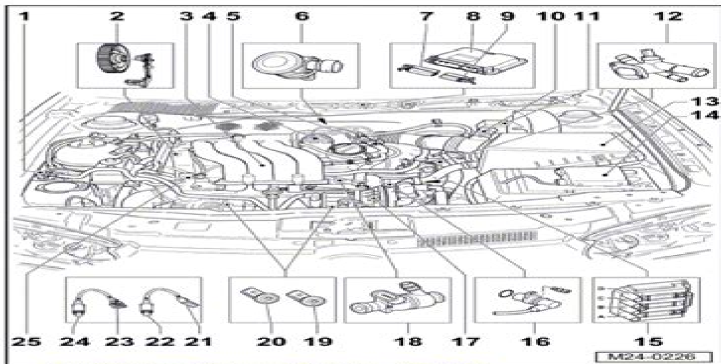
Engine Compartment Components Overview – AVH or AZG
