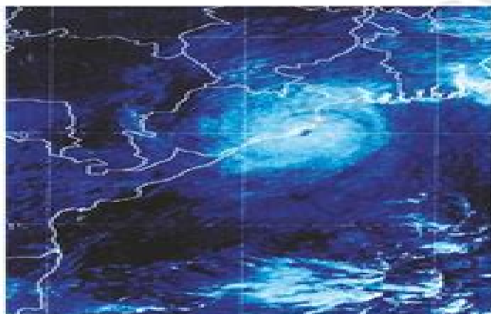
Fig. 8.1 Image taken by a satellite of a cyclone approaching the coast of Orissa
