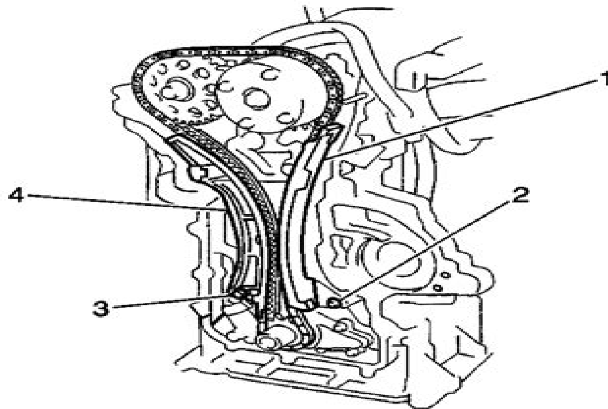
Fig. 25: Timing Chain Components Courtesy of GENERAL MOTORS CORP.
