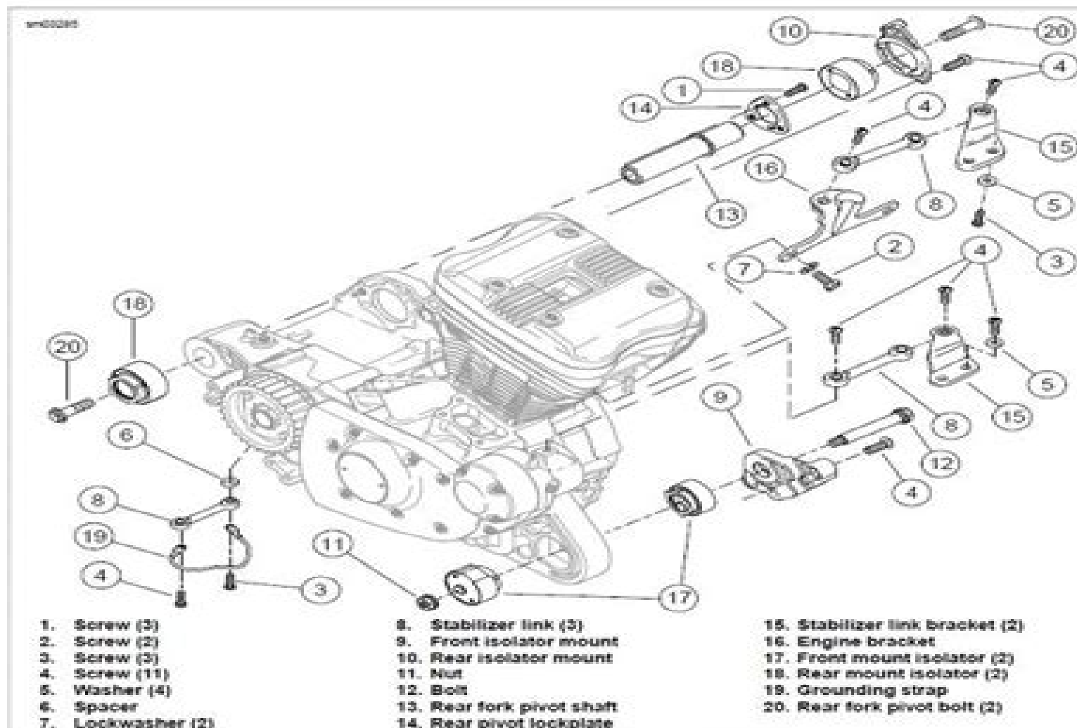
Figure 1-66. Engine Mounting Assemblies: All Models (typical)
