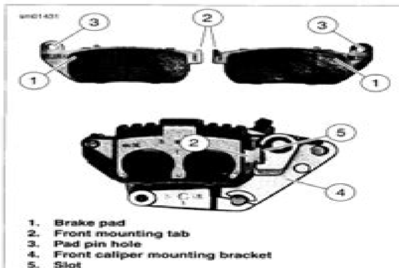
Figure 1-25. Front Brake Pads
