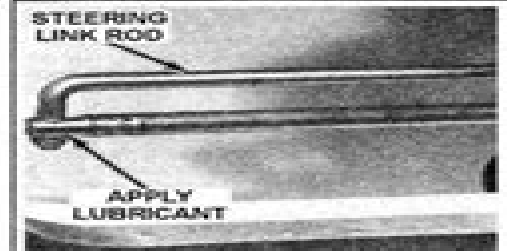
Fig. 13 Apply Yamaha All Purpose Grease to the steering link rod joint
