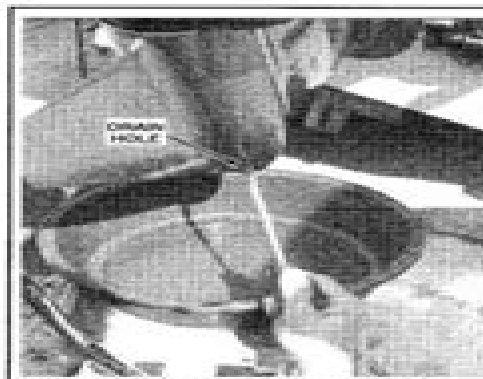
Fig. 22 When draining the lower unit, ensure it is fully tilted and a drain pan of adequate capacity is placed to catch the lubricant
