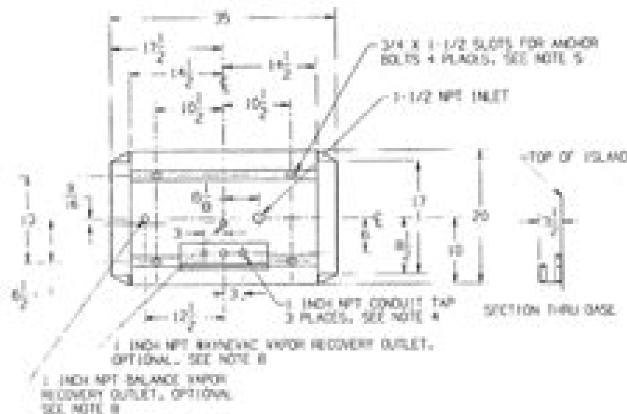
BASE DIMENSIONS
