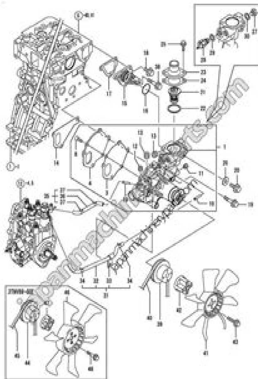
Fig.11. COOLING WATER SYSTEM
