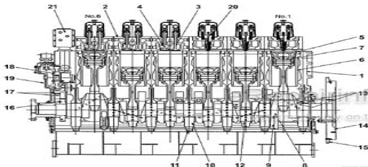
Fig. 00-04-3 Sectional View of Longitudinal
