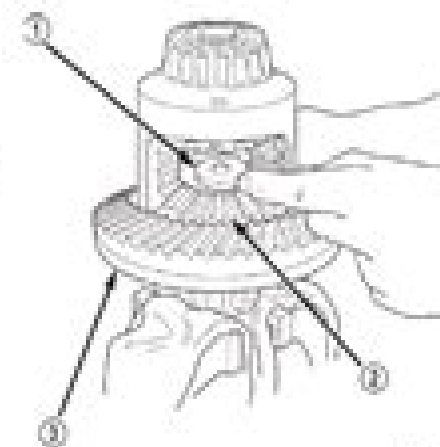
Fig. 48 Step Plate Tool Installation
