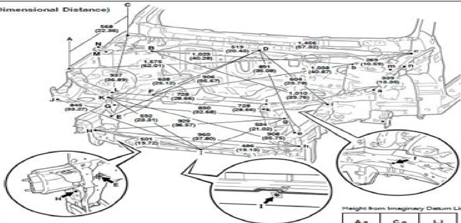
Vehicle Dimensions
