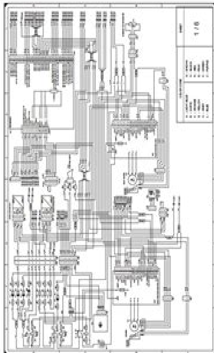
WIRING DIAGRAMS (05-8FBM26T/05-8FBMK26T/05-8FBM25T/05-8FBMK30T/ 05-8FBM30T/05-8FBM35T - Standard version)
