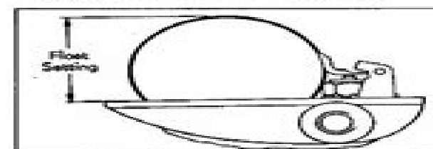
Fig. 15 FLOAT SETTING
